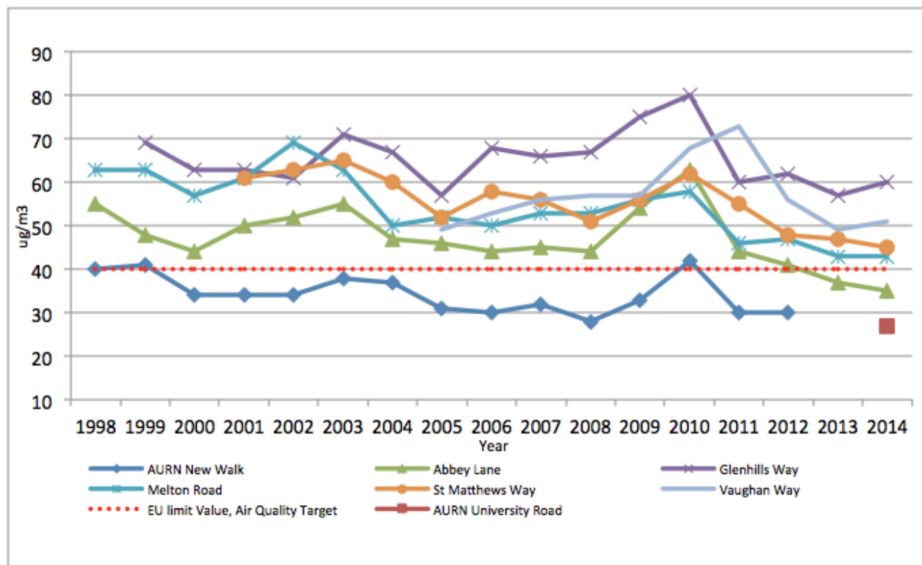
Figure 4 Leicester Air Quality Data - Annual Mean NO 2 ug/m 3
