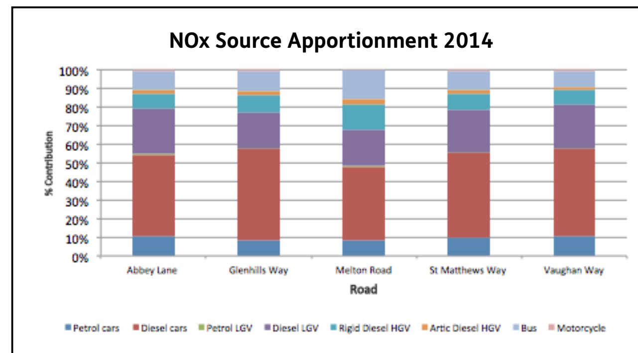
Figure 3: NOx Source Apportionment 2014
